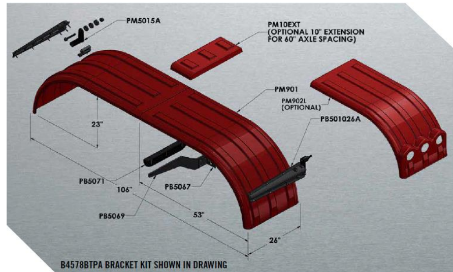
B4578BTPA BRACKET KIT SHOWN IN DRAWING
